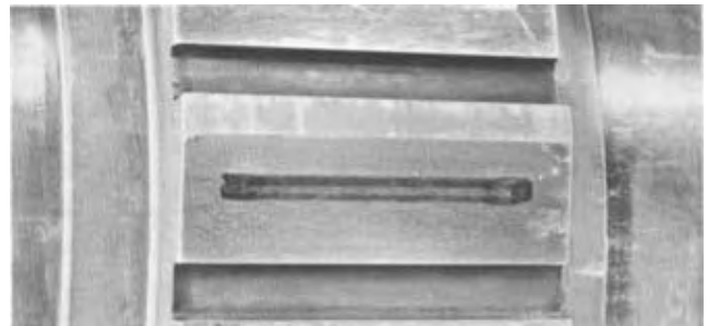
FIG. 2.49 (2342-24C) GRINDING CRACKS
