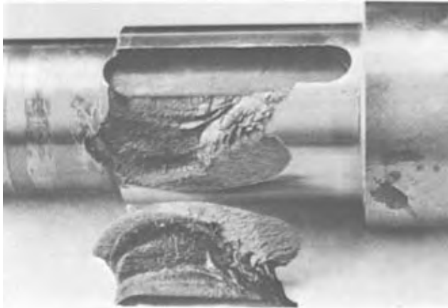
FIG. 3.5 (548-6) SHAFT FAILURE (PEELING)
