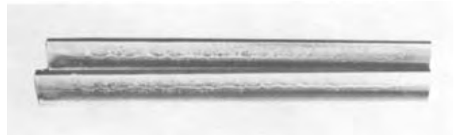
FIG. 2.28 (2342-11C) ADHESIVE WEAR (THRU HARDENED GEAR)
