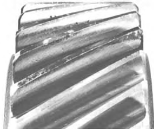
FIG. 2.3 (683-2) INITIAL (CORRECTIVE) PITTING
