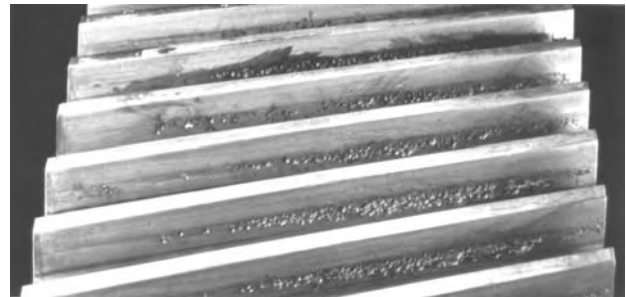
FIG. 2.10 (2342-4C) NORMAL DEDENDUM WEAR
