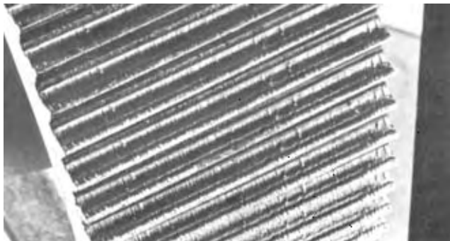
FIG. 2.24 (747-1) EXCESSIVE WEAR
