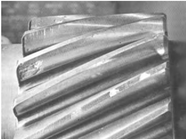
FIG. 2.17 (828-2) SPALLING (SURFACE HARDENED GEAR)
