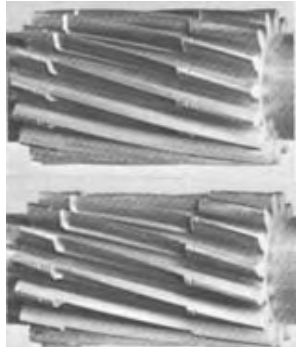
FIG. 2.26 (749-1) ABRASIVE WEAR (THRU HARDENED GEAR)
