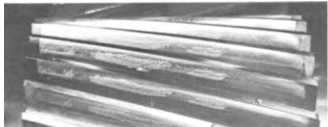
FIG. 2.29 (2342-12C) ADHESIVE WEAR (SURFACE HARDENED GEAR)
