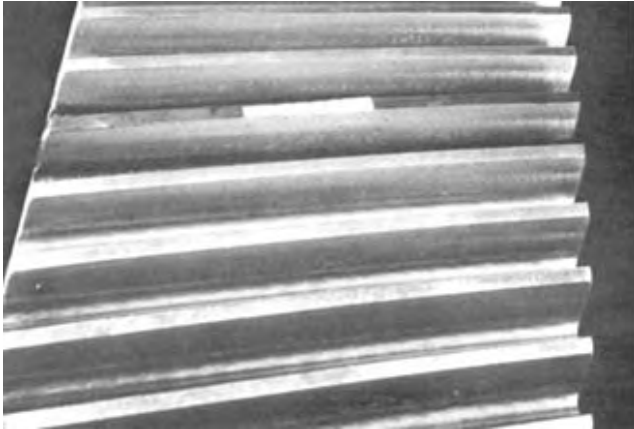
FIG. 2.21 (697-7) INITIAL PITTING AND LIGHT WEAR
