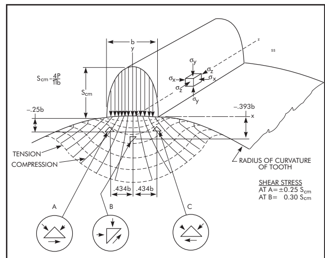
FIG. 2.1 (312-10) HERTZIAN STRESSES
