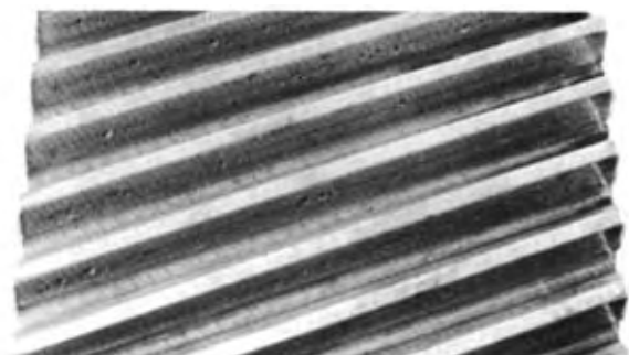
FIG. 2.5 (697-4) INITIAL (CORRECTIVE) PITTING
