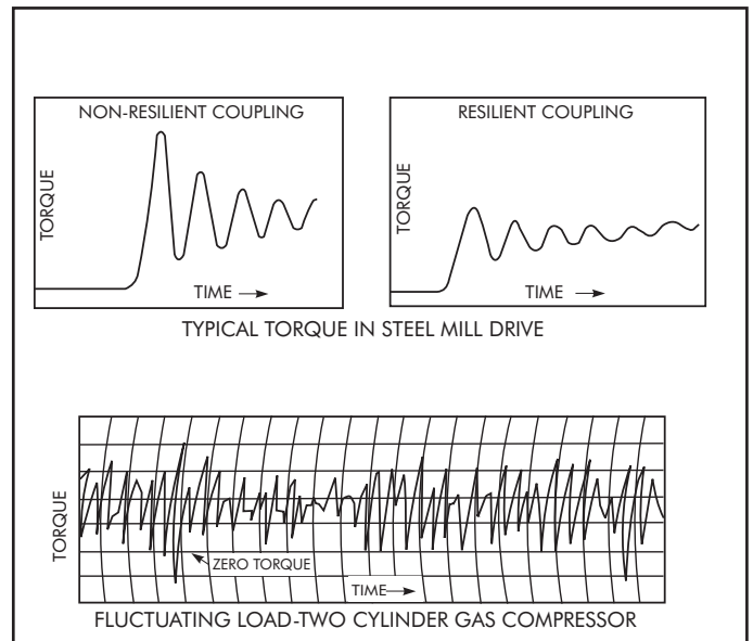
FIG. 1.2 (253-1) TORQUE METER RECORD
