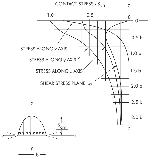
FIG. 2.2 (312-6) VARIATION OF STRESS BELOW SURFACE
