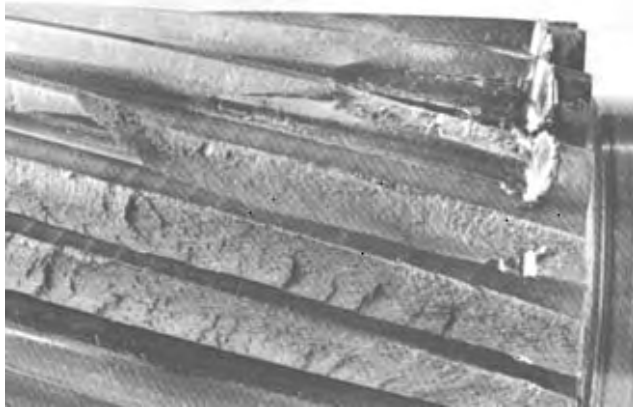
FIG. 2.41 (683-7) TOOTH FRACTURE (LOW CYCLE FATIGUE)
