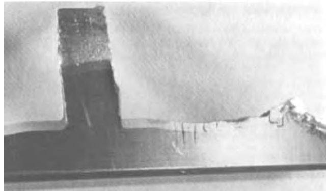
FIG. 4.7 (2342-34C) CRACKS IN CAGE FROM NOT REMOVING SHARP EDGE
