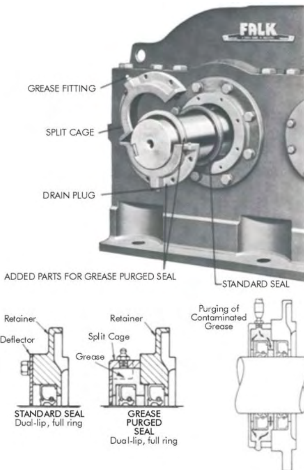
FIG. 5.1 (2342-36C) SEAL ARRANGEMENT
