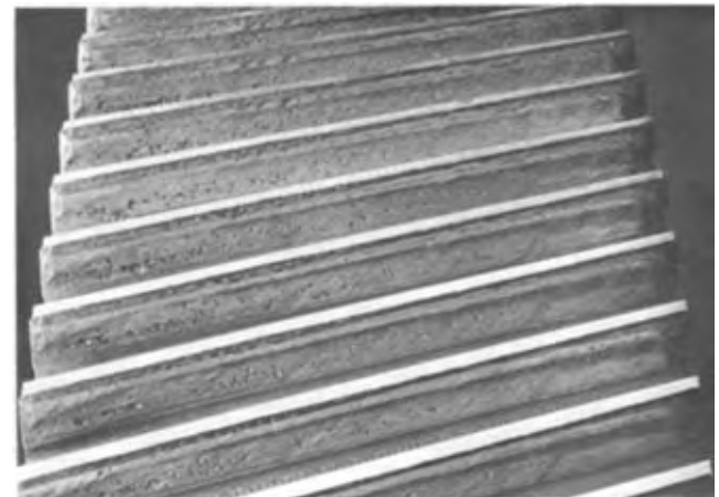
FIG. 2.37 (683-11) PLASTIC FLOW (PEENING)
