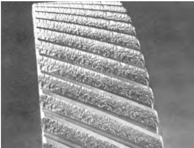
FIG. 2.25 (942-3) ABRASIVE WEAR (THRU HARDENED GEAR)
