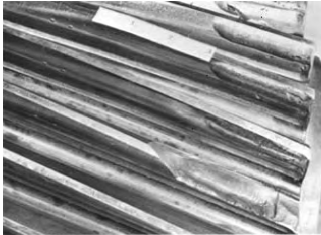
FIG. 2.33 (2342-14C) SURFACE BUMPS
