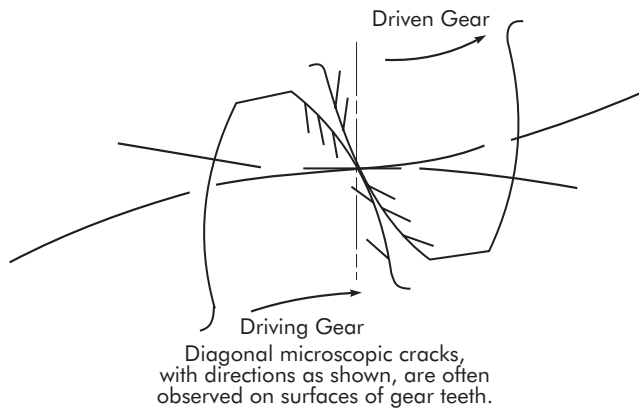
FIG. 2.12 (2342-5C) TOOTH SURFACE MICROCRACKS
