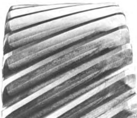
FIG. 2.13 (683-12) MICRO-PITTING (FROSTING)
