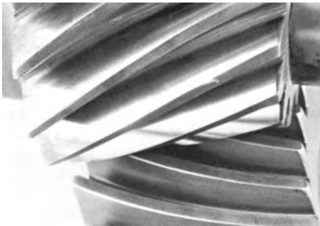
FIG. 2.22 (2342-9C) POLISHING (SURFACE HARDENED GEAR)
