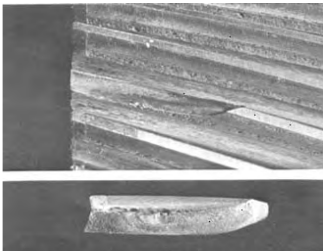
FIG. 2.42 (697-9) FATIGUE FRACTURE EMANATING FROM PIT
