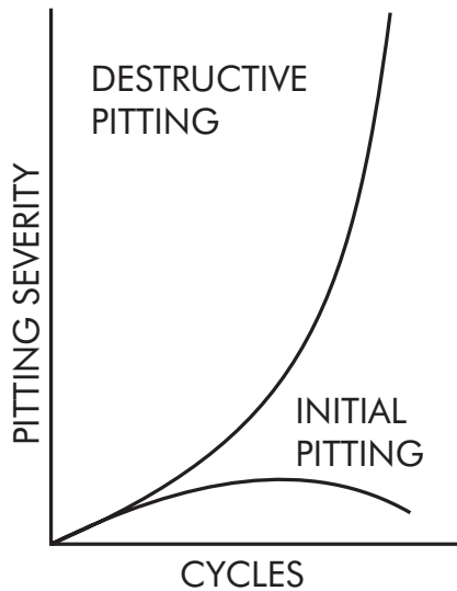
FIG. 2.6 (2342-1C) PITTING SEVERITY
