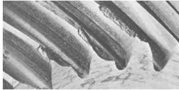
FIG. 2.43 (2342-19C) TIP CHIPPING (THRU HARDENED GEAR)
