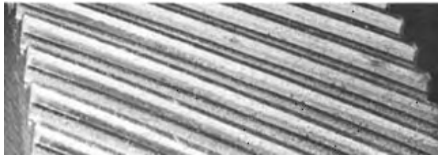
FIG. 2.23 (697-10) TYPICAL TOOTH SURFACE APPEARANCE
