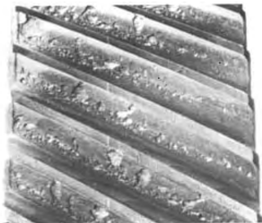
FIG. 2.7 (828-1) DESTRUCTIVE (PROGRESSIVE) PITTING THRU HARDENED GEARS
