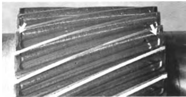
FIG. 2.34 (2342-15C) WEAR PADS
