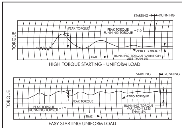
FIG. 1.1 (253-2) TORQUE METER RECORD
