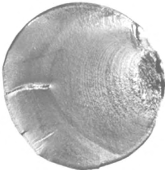
FIG. 3.1 (2342-25C) BENDING FRACTURE
