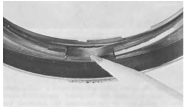
FIG. 5.7 (2342-42C) RADIAL AND CIRCUMFERENTIAL CRACKS DUE TO OZONE
