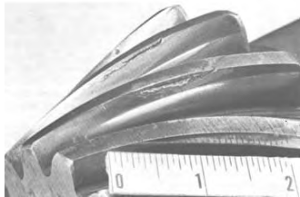
FIG. 2.44 (2342-20C) TIP CHIPPING (SURFACE HARDENED GEAR)
