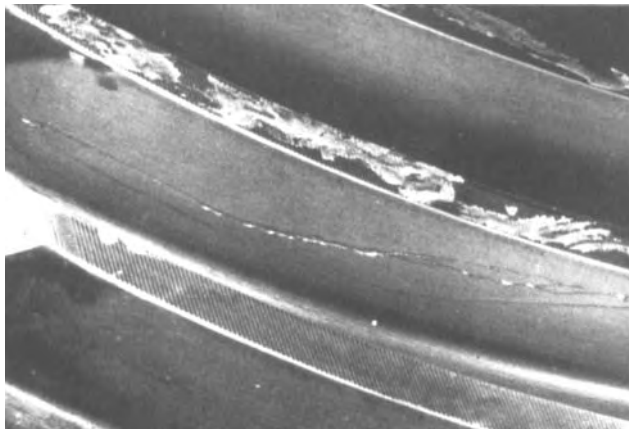
FIG. 2.18 (2342-8C) CASE CRUSHING
