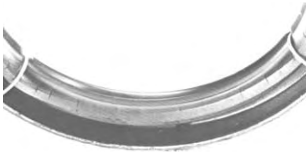
FIG. 5.4 (2342-39C) HEAT CRACKING
