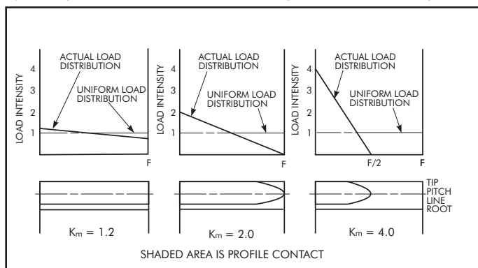
FIG. 1.3 (253-3) CONTACT PATTERNS AND LOAD DISTRIBUTION
