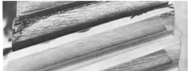
FIG. 2.27 (2342-10C) SCRATCHING
