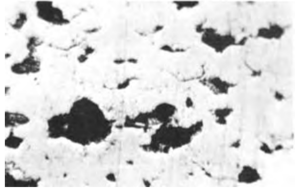
FIG. 2.14 (2342-6C) MICRO-PITTING (ENLARGED PHOTO)
