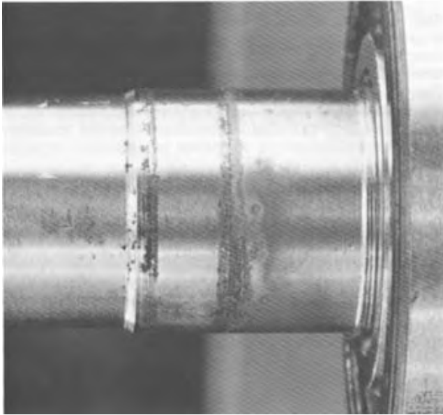
FIG. 5.8 (2342-43C) JOURNAL WEAR
